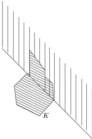
Figure 2: Fundamental domain for the action of L
