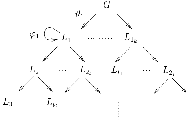
Figure 1: M-R diagram
