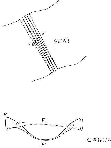
Figure 6: Shortening of the annulus F
