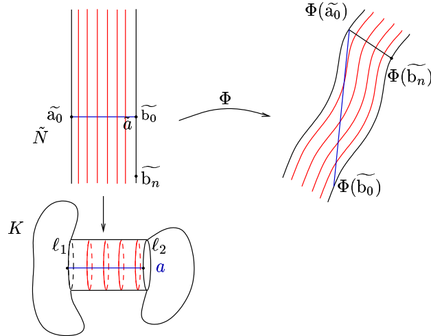
Figure 4: Shortening the simplicial component
