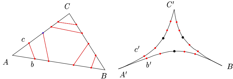
Figure 3: Defining the lamination \tilde{\Lambda}_f on \tilde{K}
