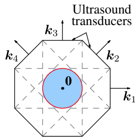
FIG. 1. Each parallel pair of ultrasound transducers establishes an ultrasound wave that is close to a plane wave in the rectangle delineated by the dotted lines perpendicular to the ultrasound transducers. The plane wave model Eq. (2) accurately represents the ultrasound wave field generated by this transducer arrangement in the blue region. The red circle indicates the region we evaluate.
